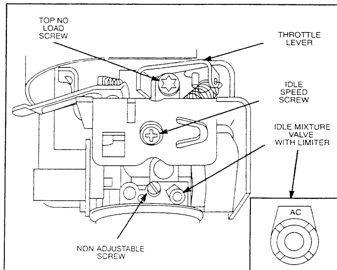
Carburetor adjustments
